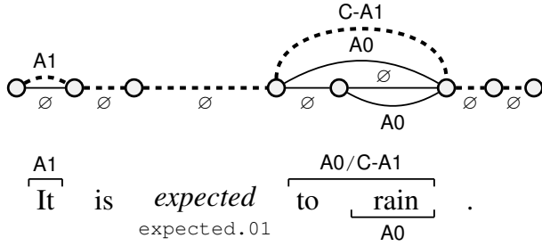
Figure 3: Lattice corresponding to the dynamic program for the no span overlap constraint. The path of the correct argument assignment is indicated with dashed edges.
