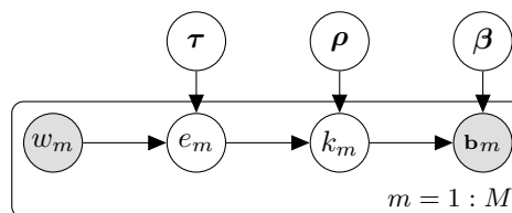
Figure 1: Selective context model. The mention phrase w_m provides a prior distribution over possible entities for mention m . The latent variable k_m selects a relevant context feature b_{m,k_m} that fires for entity e_m ; the remaining features are drawn from a background distribution p(b_j|\beta_j) . The entity is represented as a latent variable here, but it is observed for the labeled training mentions.
