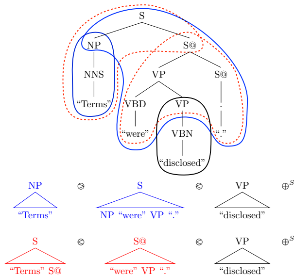
Figure 4: Above: an example of a set of fragments extracted from the tree in Figure 1. Below: two incremental derivations that generate it. Colors (and lines strokes) indicate which derivation fragments belong to.
